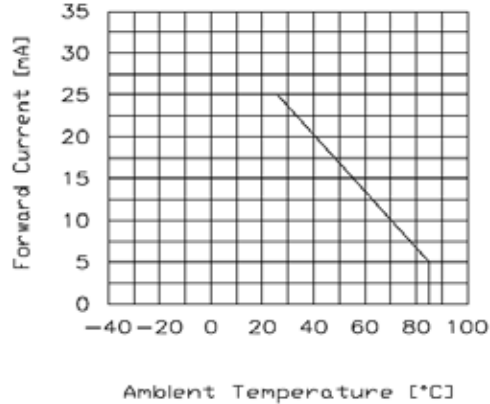
Fig 6. Maximum allowable dc current per segment vs. A function of ambient temperature
